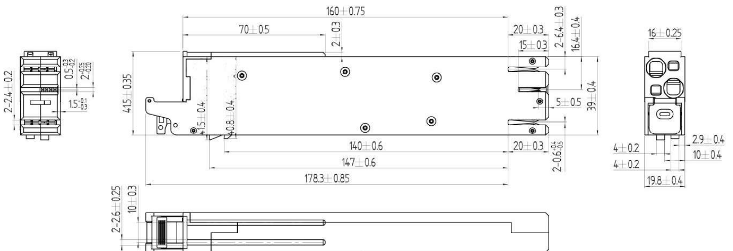
MB8Z-63 Outline and installation dimensions
