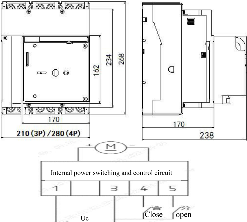
Wiring diagram for electric operation
