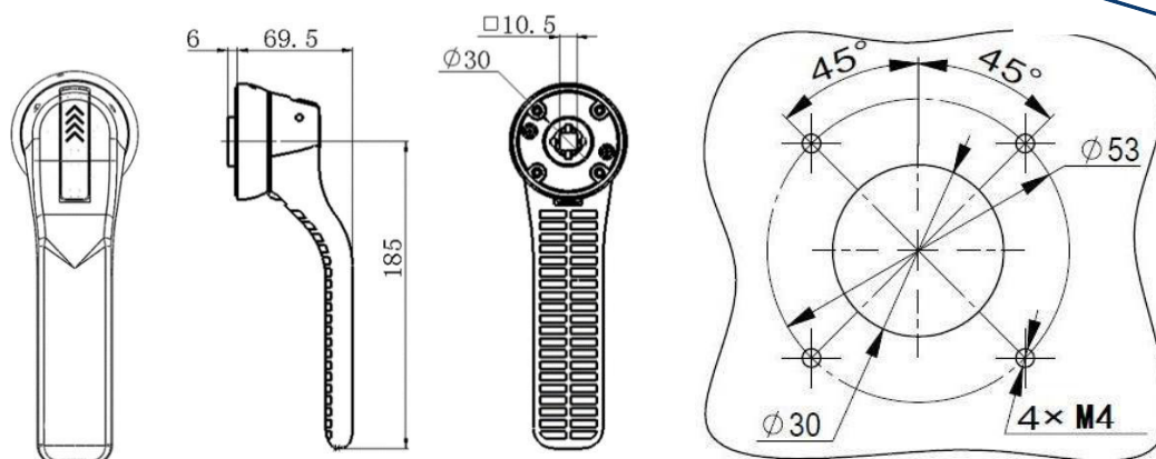
Handle Mounting Hole Diagram
