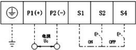
Schematic diagram of electrical operation wiring
