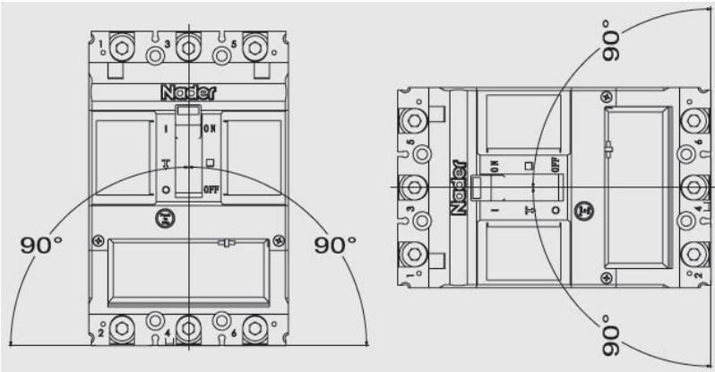
Vertical Installation
