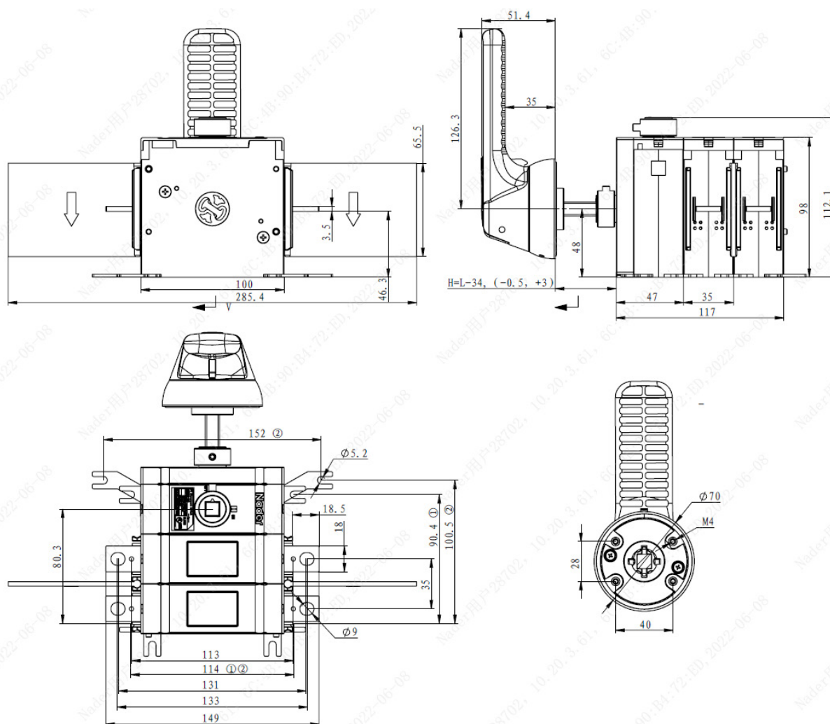
Side operation outline installation drawing
