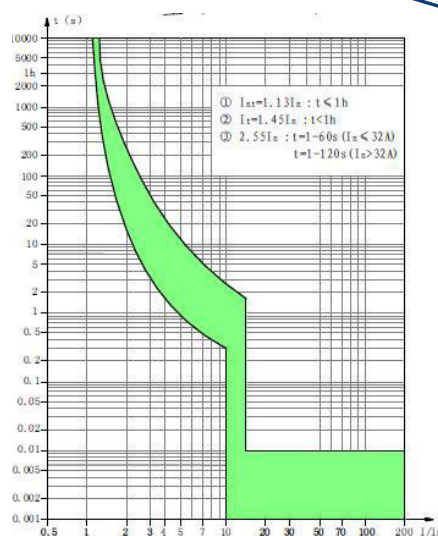
D Curve
